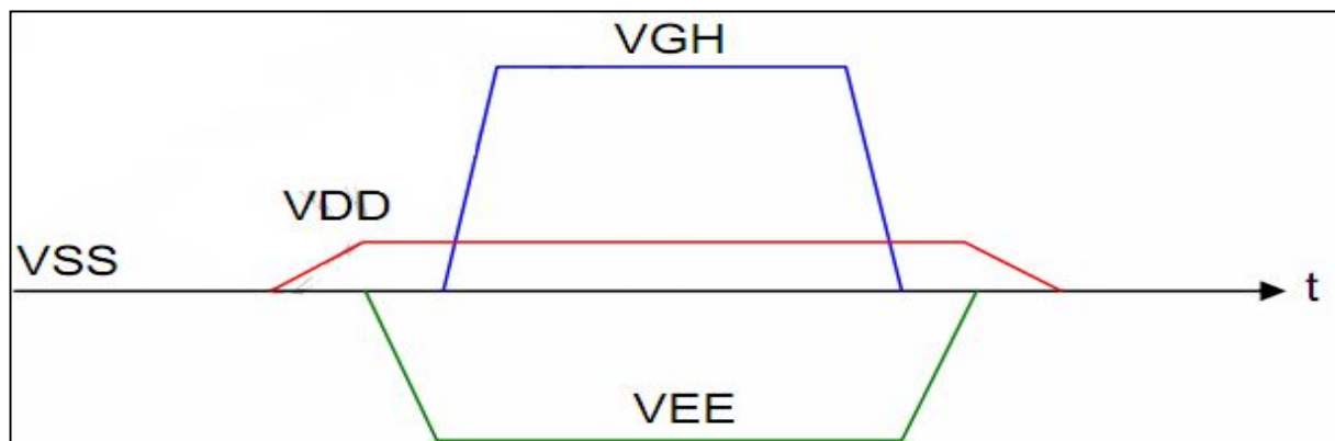
Figure 5.7 Gate Power On/Off Timing Sequence
