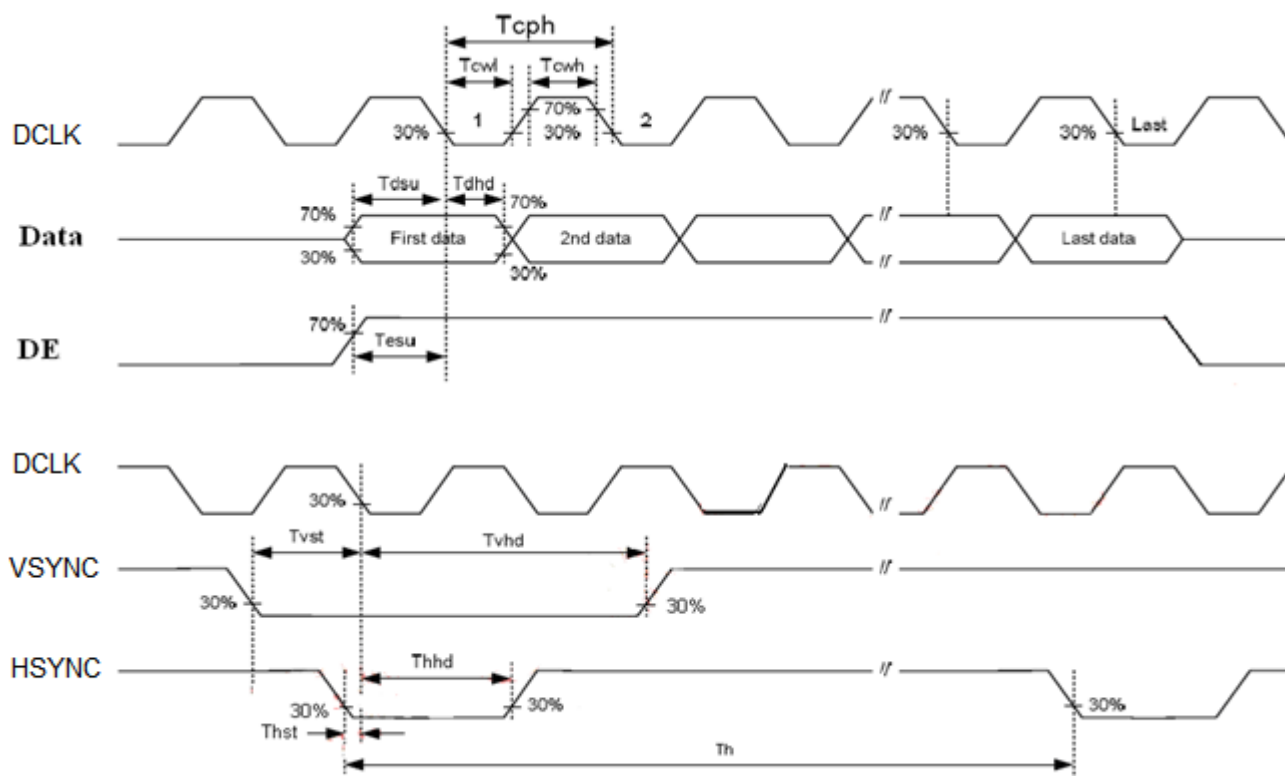
Figure 6.1 AC characteristics
